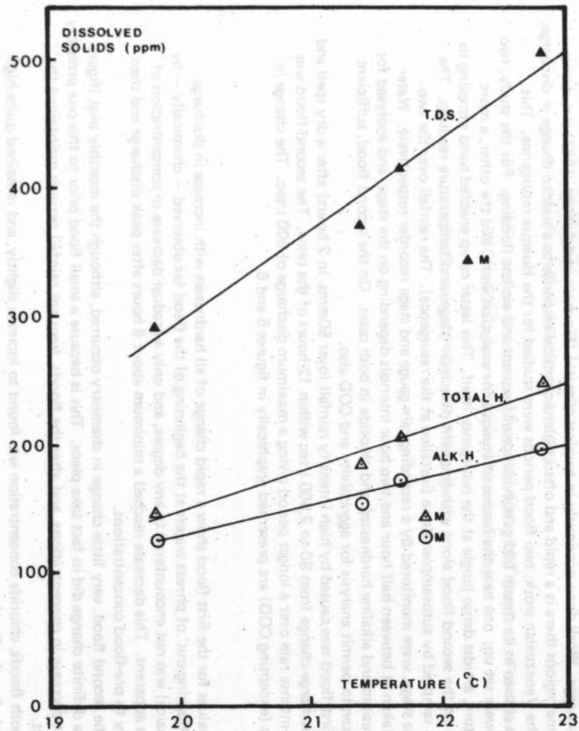
Fig. 4. The Relationship between Hardnesses, Dissolved Solids and Temperature, for resurgences.
