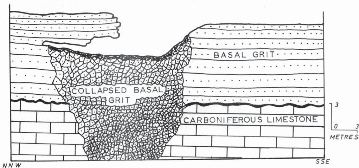
Fig. 8. Section across a small open cave in Basal Grit on the dip slope of Gwaen Cefn-y-gareg (Grid. Ref. 942134), near Ystradfellte.
