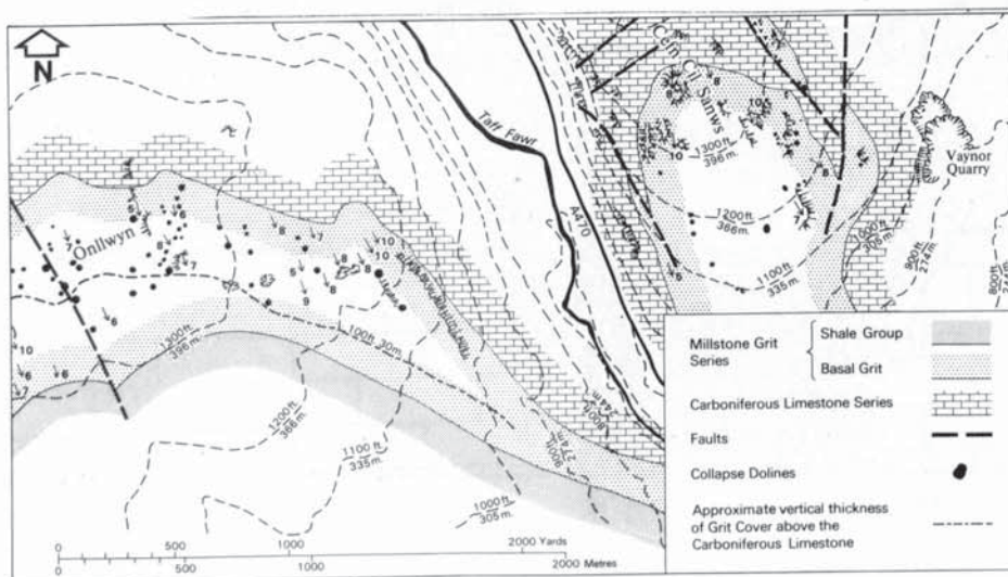
Fig. 10. Solution subsidence phenomena on the Basal Grit outcrops of the upper Taf Fawr valley area.
