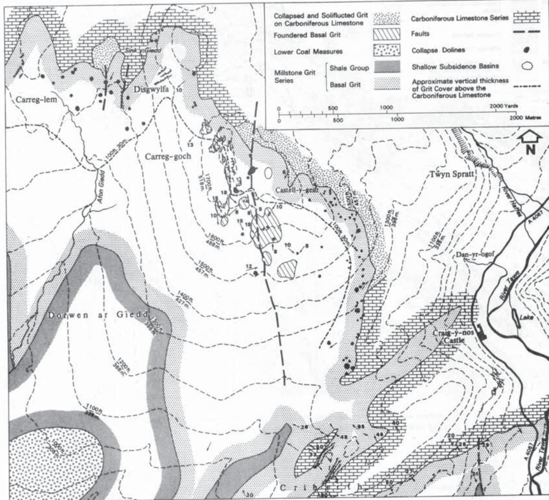
Fig. 5. Solution subsidence phenomena on the Basal Grit outcrop of the area lying between Black Mountain and the Upper Tawe Valley.
