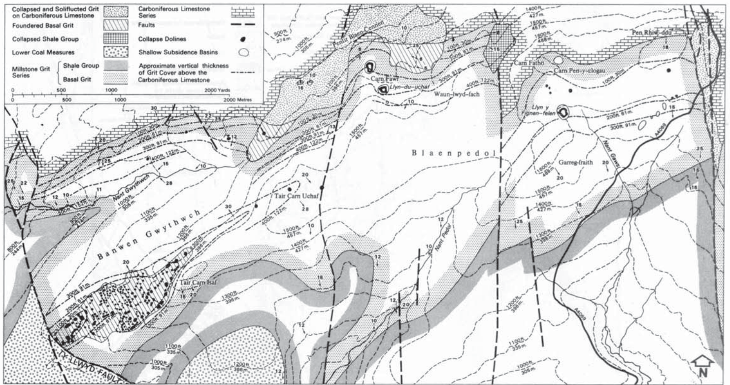
Fig. 3. Solution subsidence phenomena on the Basal Grit outcrop of the Black Mountain area lying west of the Brynamman - Llangadock road (A. 4069).
