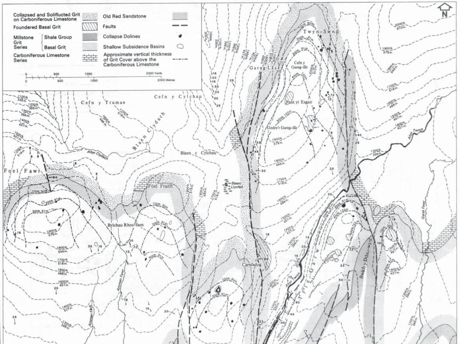
Fig. 4. Solution subsidence phenomena on the Basal Grit outcrop of the Black Mountain area lying east of the Brynamman - Llangadock Road (A. 4069).
