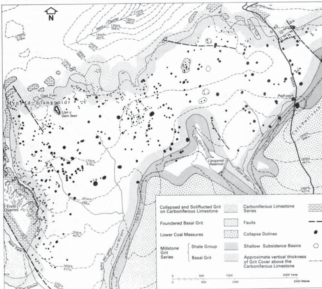
Fig. 12. Solution subsidence phenomena on the Basal Grit, Middle Shales outcrops of Mynydd Llangynidr.
