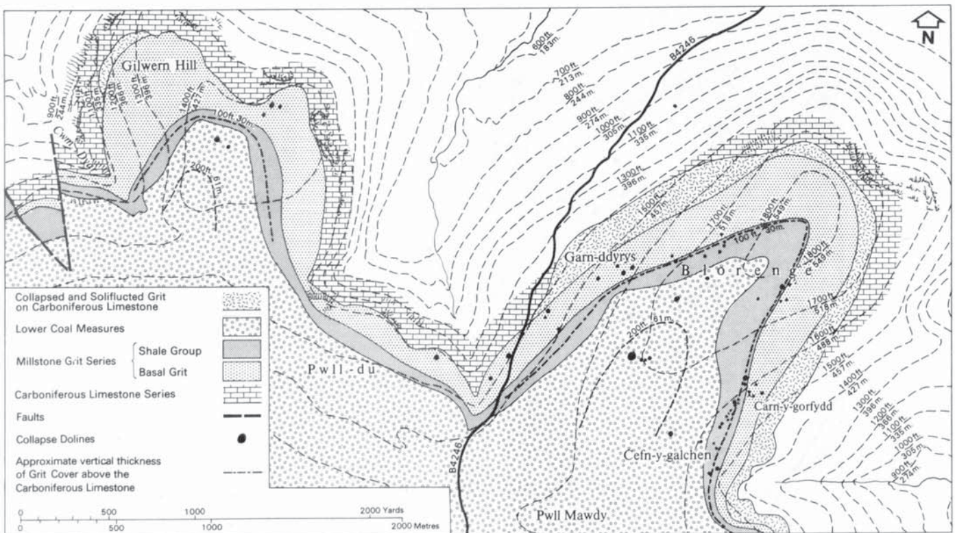
Fig. 14. Solution subsidence phenomena on the Basal Grit, Middle Shales and Lower Coal Measure outcrops of Gilwern Hill and the Bloreng.
