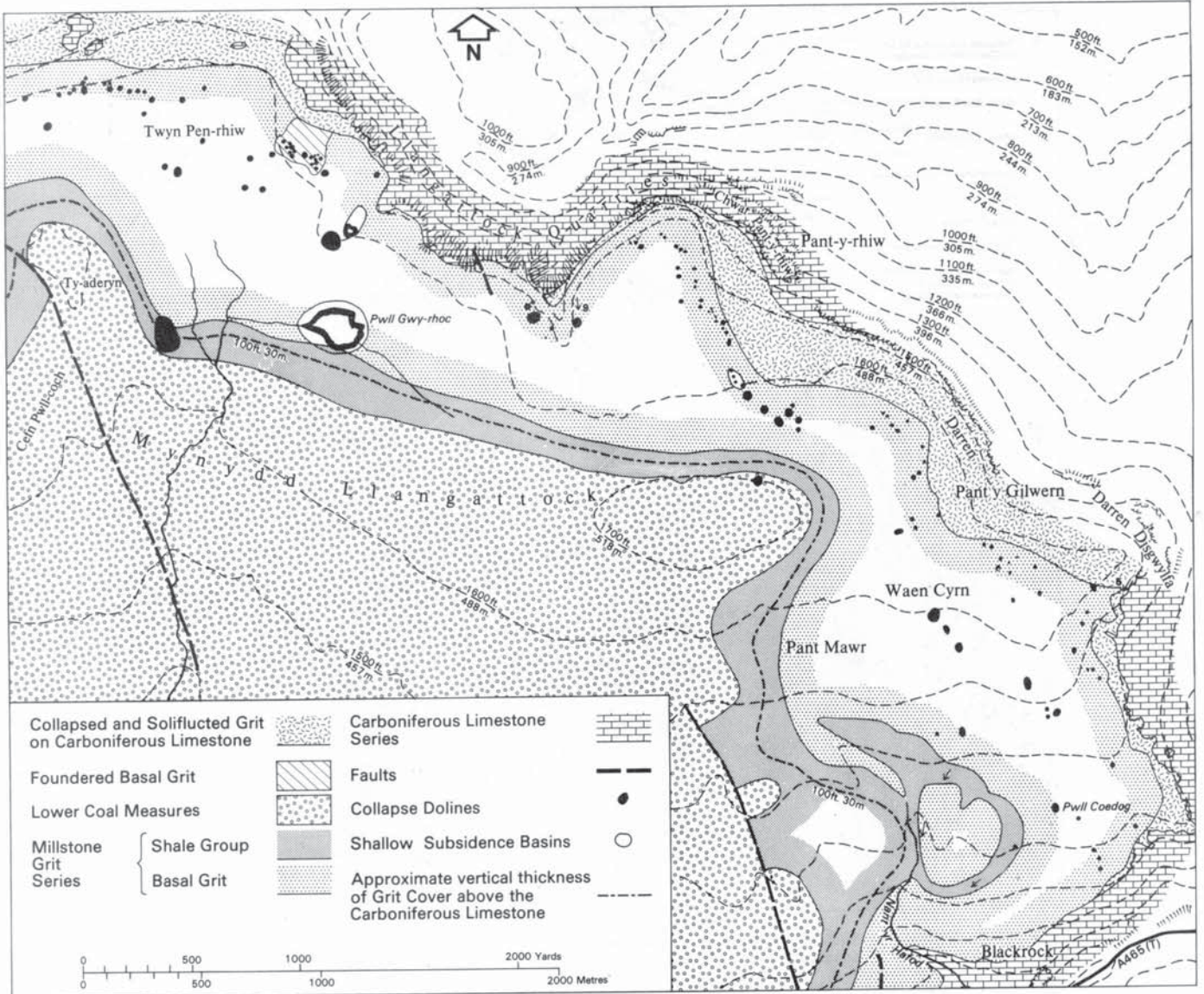
Fig. 13. Solution subsidence phenomena on the Basal Grit, Middle Shales and Lower Coal Measure outcrops of Mynydd Llangatwg.
