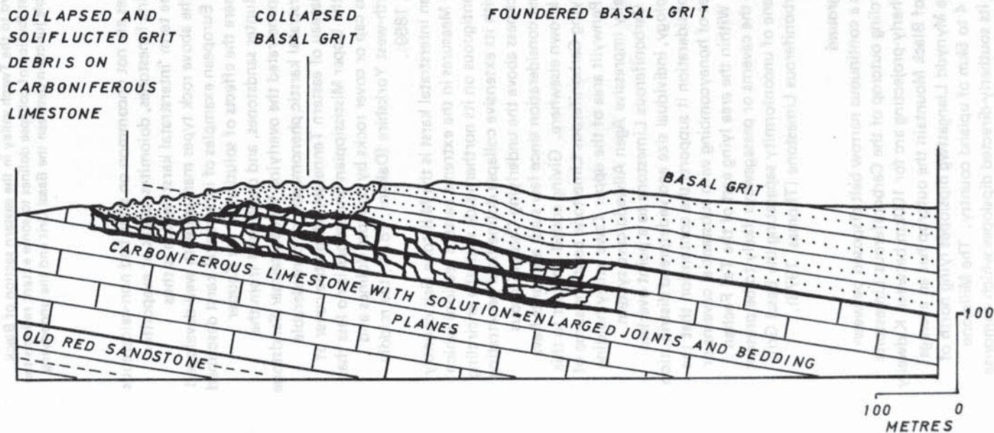
Fig. 2. Schematic section illustrating collapsed and soliflucted Millstone Grit residue on the Carboniferous Limestone, subsided Millstone Grit and foundered Grit beds.
