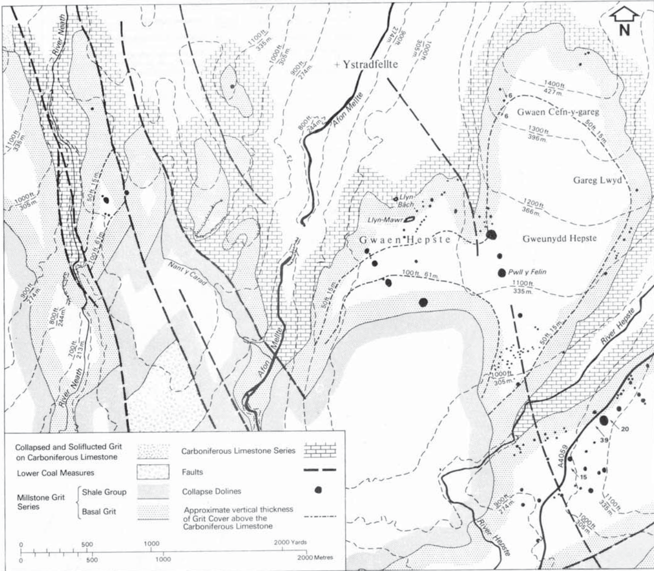
Fig. 7. Solution subsidence phenomena on the Basal Grit outcrops of the Ystradfellte area.
