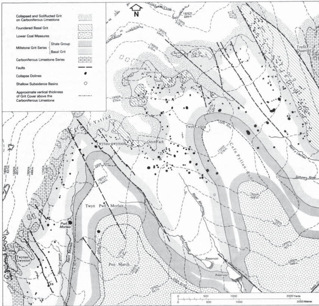
Fig. 11. Solution subsidence phenomena on the Basal Grit, Middle Shales and Lower Coal Measures outcrops of the Taf Fechan to Trefil area.
