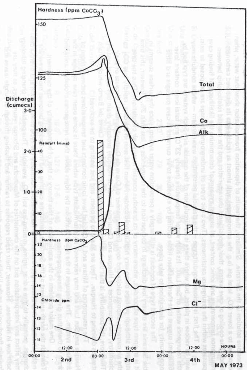
Fig. 5. Chemistry and Discharge changes for the first flood (May '73) of the Hueque resurgence.
