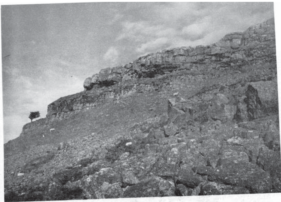
9. The western scarp edge of Gwaen Cefn-y-gareg, near Ystradfellte. The junction of the Basal Grit with the underlying Carboniferous Limestone is defined by a well-marked bedding plane cave.
