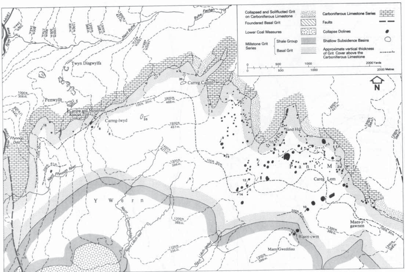
Fig. 6. Solution subsidence phenomena on the Basal Grit and Middle Shales outcrops lying between the upper Tawe and upper Neath valleys.
