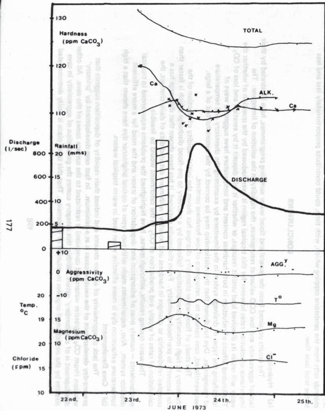
Fig. 6. Chemistry and Discharge changes for the second flood (June '73) of the Hueque resurgence. (COD changes not shown).
