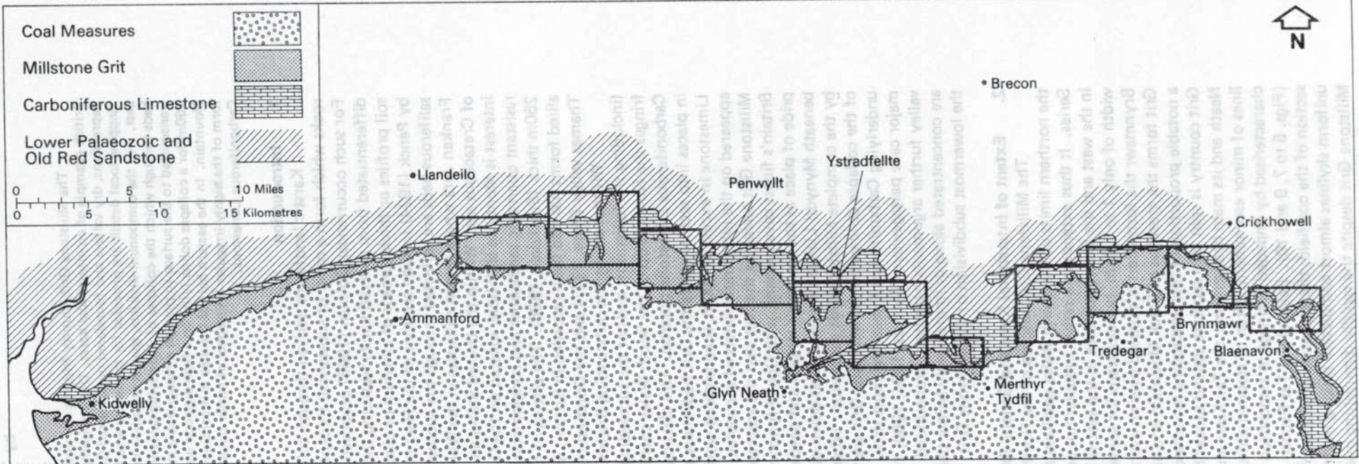
Fig. 1. Generalised geological map of the North Crop region of the South Wales coalfield showing the location of the areas subjected to detailed survey.
